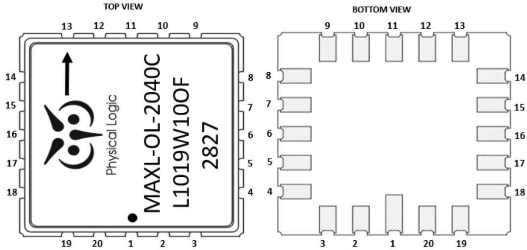
Figure 4 Pinout Description
