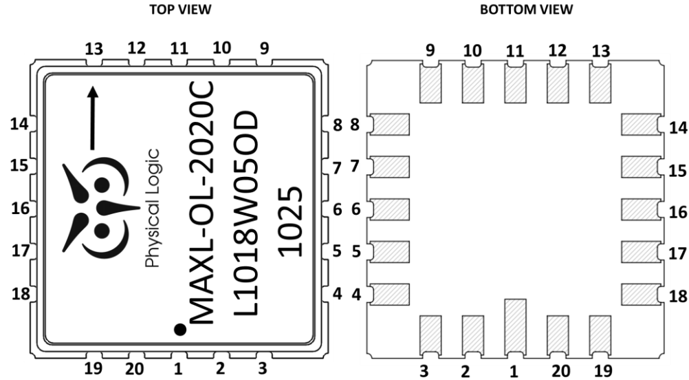
Figure 4 Pinout Description
