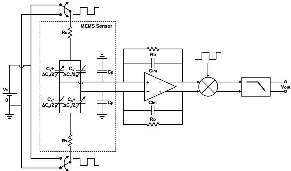
Figure 3 Simplified View of Sensor Operation
