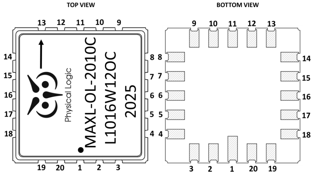
Figure 4 Pinout Description
