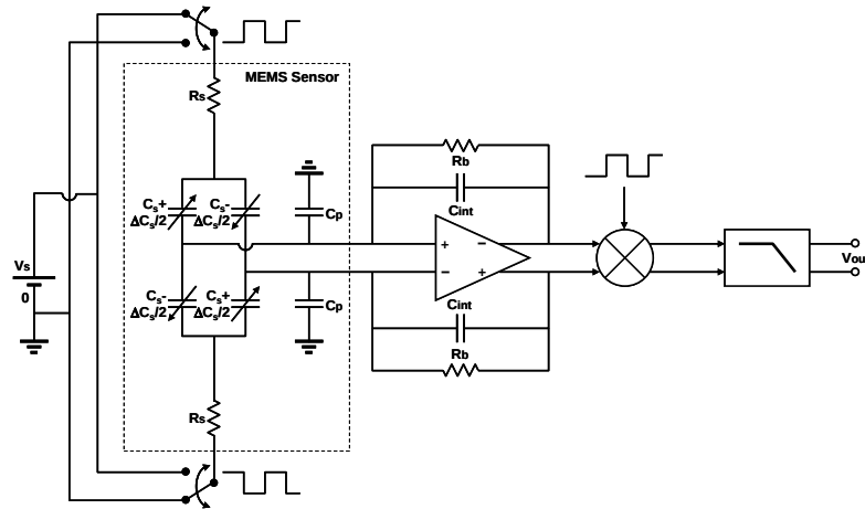
Figure 3 Simplified view of sensor interface
